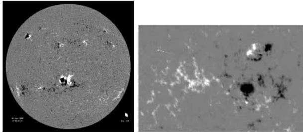
Fig. 2. (a) Sunspots in a full disk magnetogram, (b) Magnetogram around an active region
